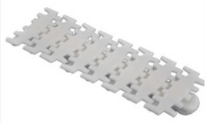
Flexible chain 103 A (POM-40C+90C) Pitch 35.5 mm.
